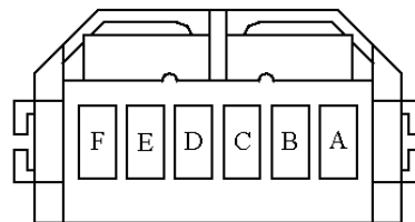
SAFETY START MODULE VIEWED FROM MATING SIDE
